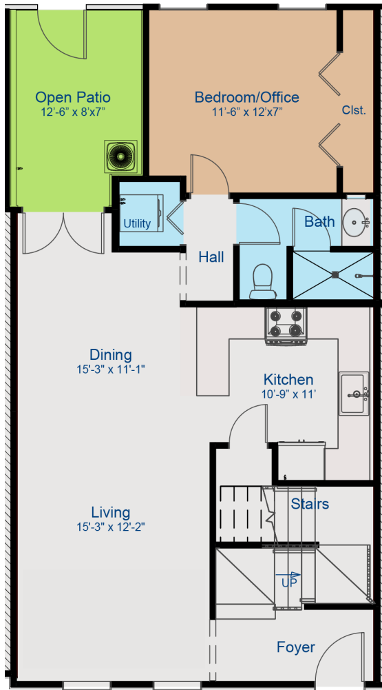
Unit 3 First Floor Plan
