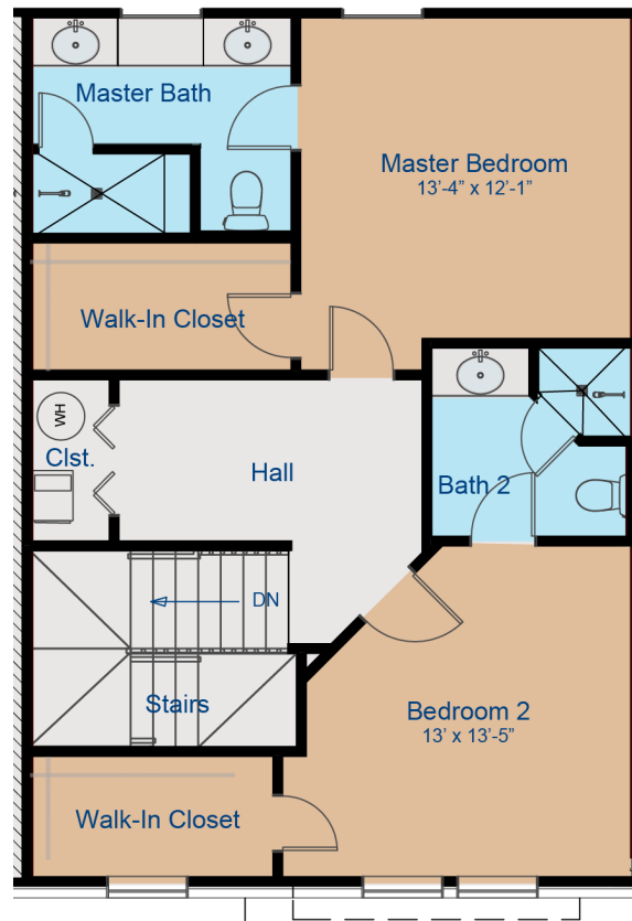
Unit 8 Second Floor Plan
