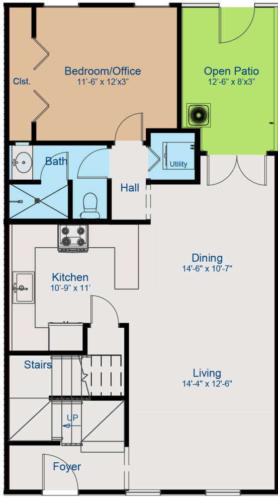
Unit 2 First Floor Plan
