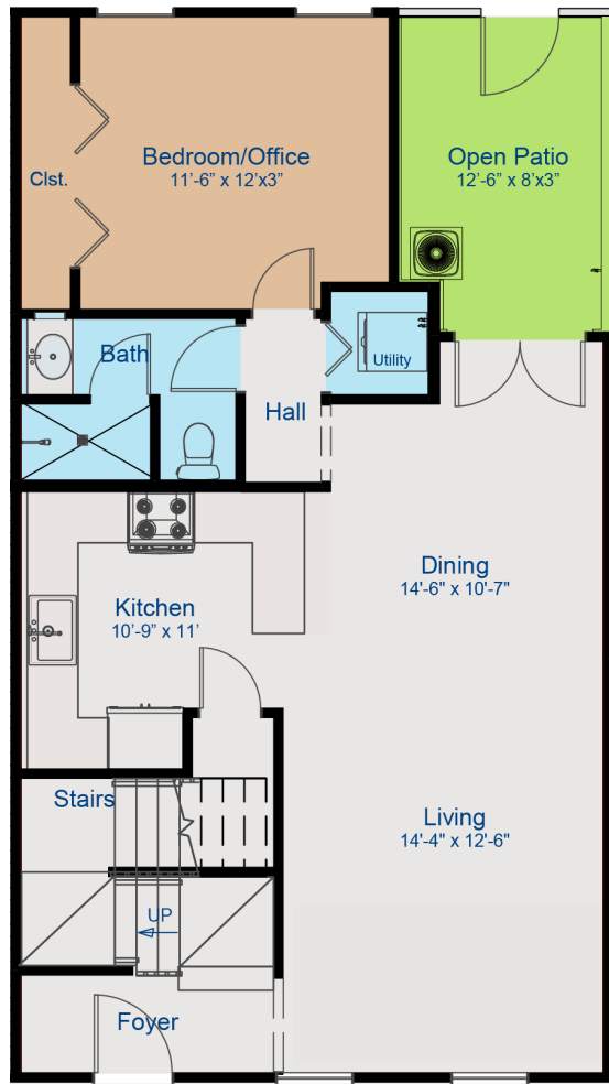
Unit 6 First Floor Plan
