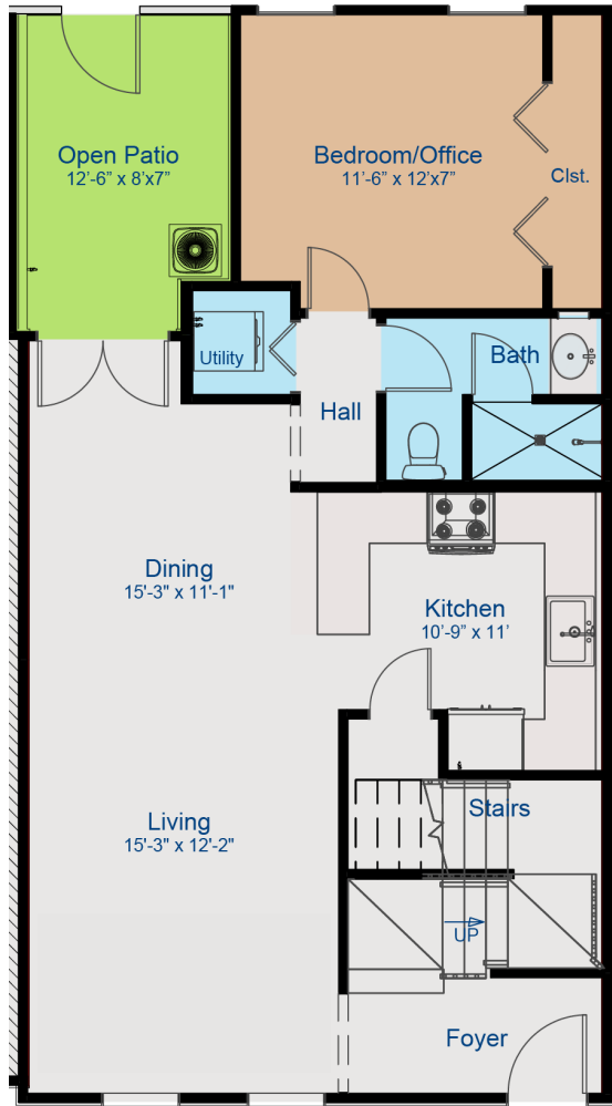
Unit 7 First Floor Plan
