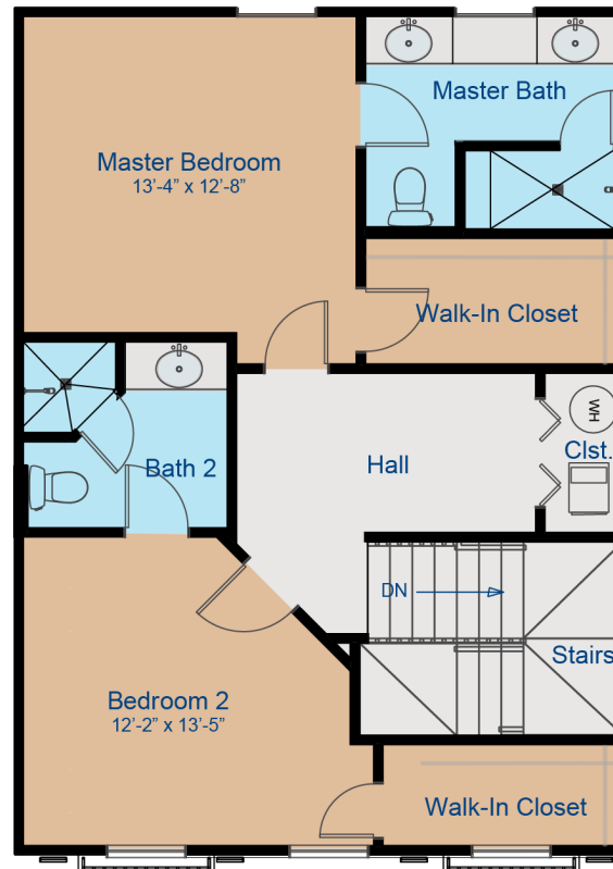
Unit 5 Second Floor Plan
